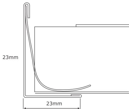
Perimeter Details
